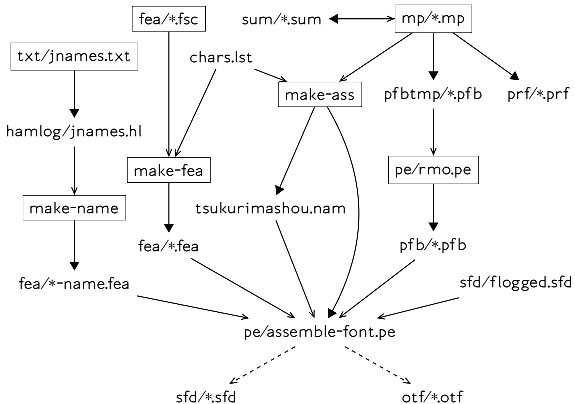
Figure 2: Building the fonts themselves. Checksums in sum/ provide fine-grained change tracking on the Metapost files in mp/ , which define Postscript “page” fonts each covering up to 256 code points. Those are processed to remove overlaps (RMO) and end up in pfb/ . The make-ass script also scans the Metapost files to get a list of defined code points and some other metadata; its main output is a FontAnvil script that assembles the page fonts into full-coverage OpenType or FontAnvil native fonts. Non-proportional fonts become OpenType and are finished here; proportional fonts become FontAnvil native and are processed further. The assemble-font script also makes use of per-family feature files from make-fea (defining things like glyph composition) and per-font feature files from make-name (defining metadata table contents). The “proof” files in prf/ are generated as a side effect of compiling the PostScript page fonts, and pass information about glyph construction to both the automatic documentation generator and the GPOS table generator.
