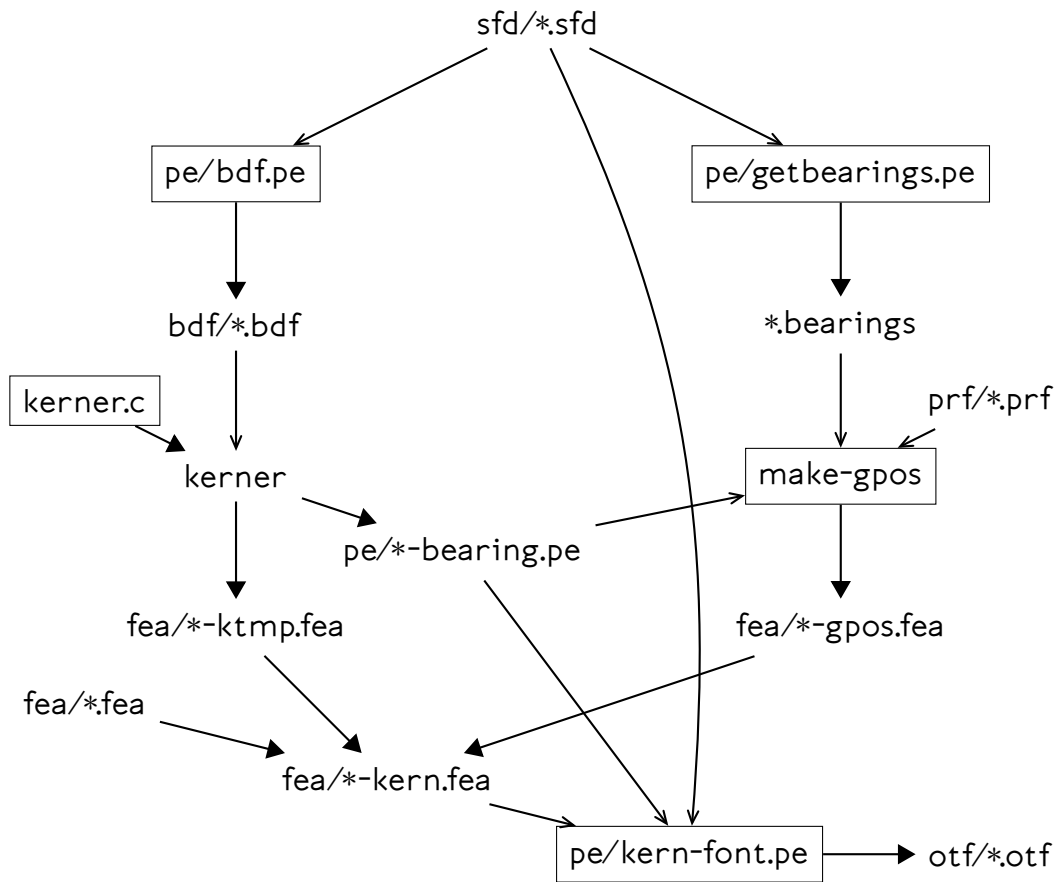
Figure 3: Additional processing for proportional fonts. The SFD file containing the font outlines is converted to a BDF bitmap font, which feeds the kerner program. That generates a “ktmp” feature file with the actual kerning data, and a FontAnvil script to apply the chosen bearings. At right, the make-gpos script reads the proof files to determine accent anchor locations. But since those must be adjusted when the bearings are set, it also needs “before” bearing information extracted by getbearings, and “after” obtained by reading the bearings script from kerner. The feature files for kerning, mark composition (GPOS), and family features are all combined and applied by the kern-font script, which runs the bearings script as a subroutine, finally producing a complete OTF font.
