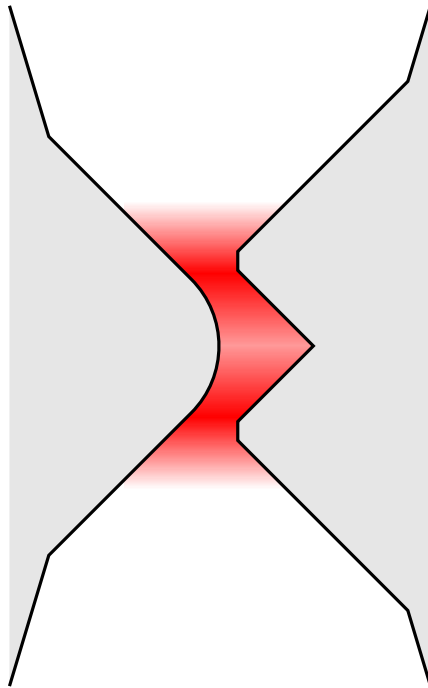
Figure 5: Closeness computation
